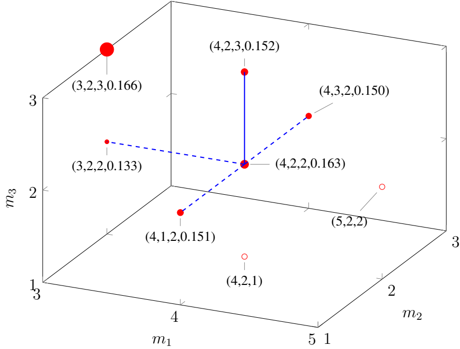
Figure 3.18: When the conventional PSO is used, the search starting from (4, 2, 2) is not able to reach the global optimum (3, 2, 3) .
